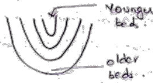
Syncline
