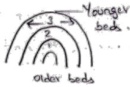
Anticline
