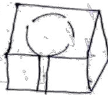
Arcuate faults
