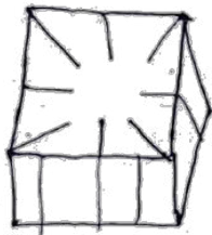
Radial faults
